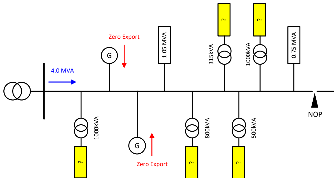
Figure A3 Allocation of Demand to HV Connections
