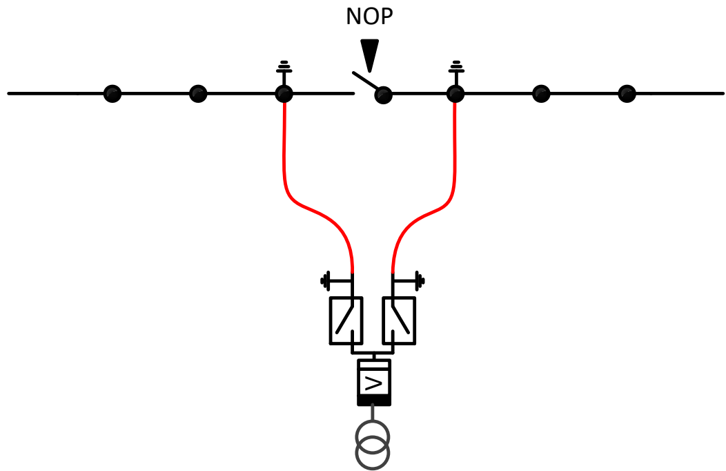
Figure 3 Connecting a Ground Mounted substation into an Overhead Line
