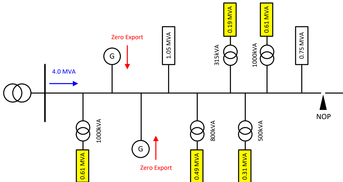
Figure A3 Allocation of Circuit Demand and remaining load to Network Substation Maximum Demands
