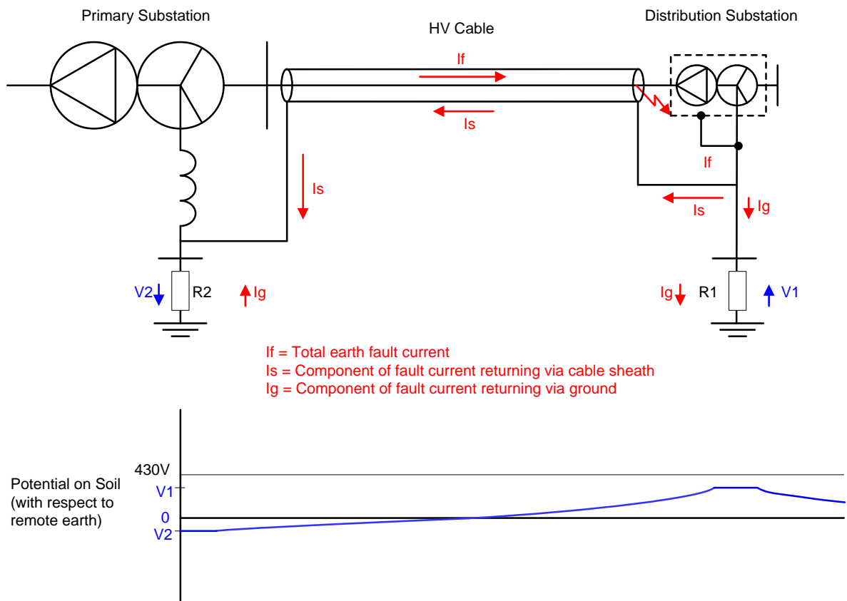
Figure 49: Rise of Potential (Cable Fed Substation)
