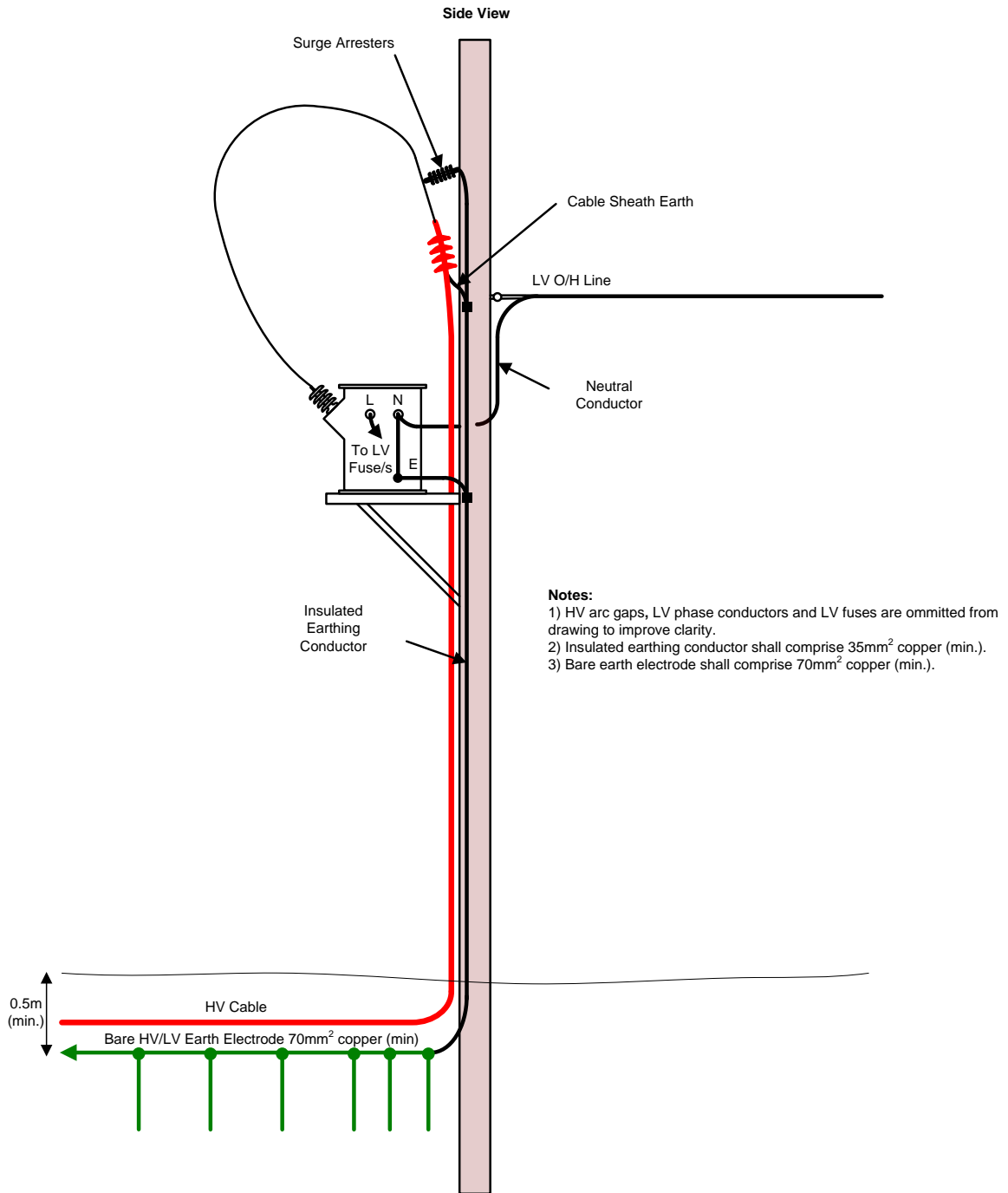
Figure 19: Combined HV and LV Earthing at Pole Mounted Substations
