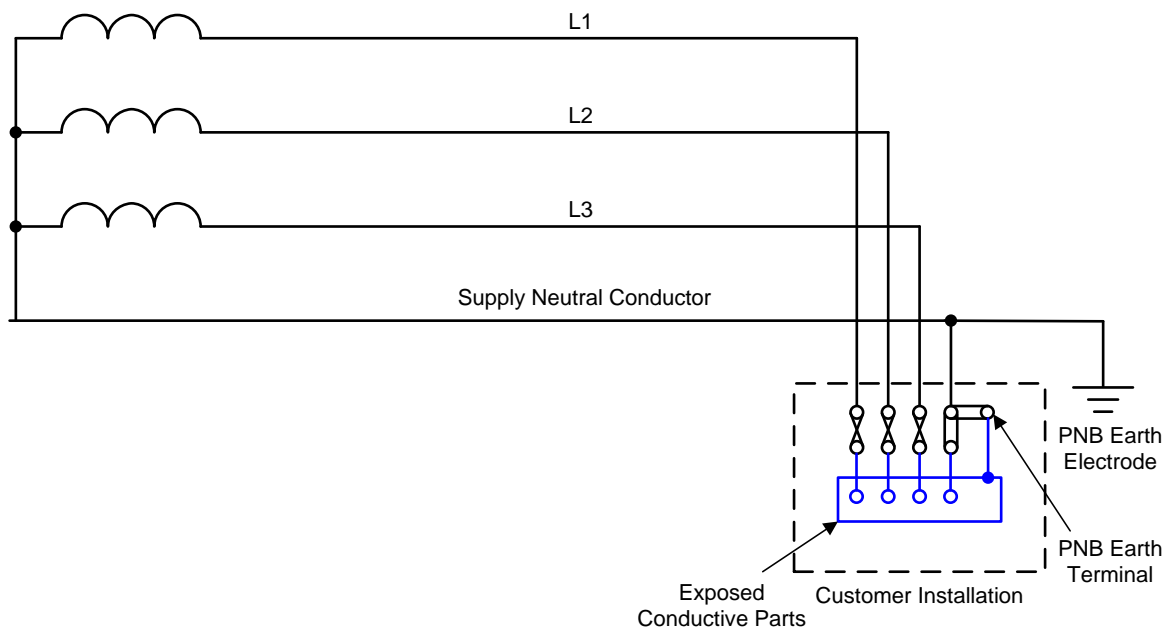
Figure 40: Protective Neutral Bonding (PNB)
