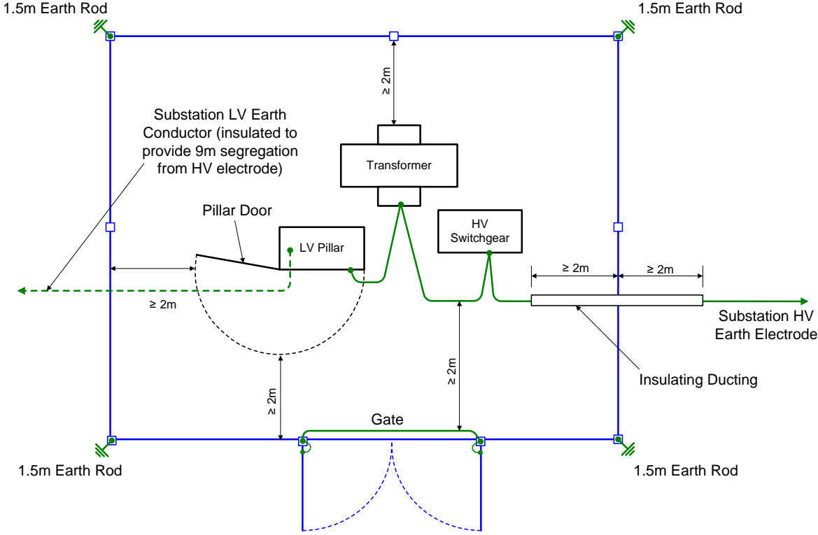
Figure 33: Independently Earthed Metal Fencing System at Substations with Segregated HV and LV Earthing (Outdoor Arrangement)
