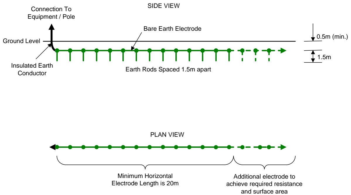
Figure 3: Earth Electrode Arrangement B
