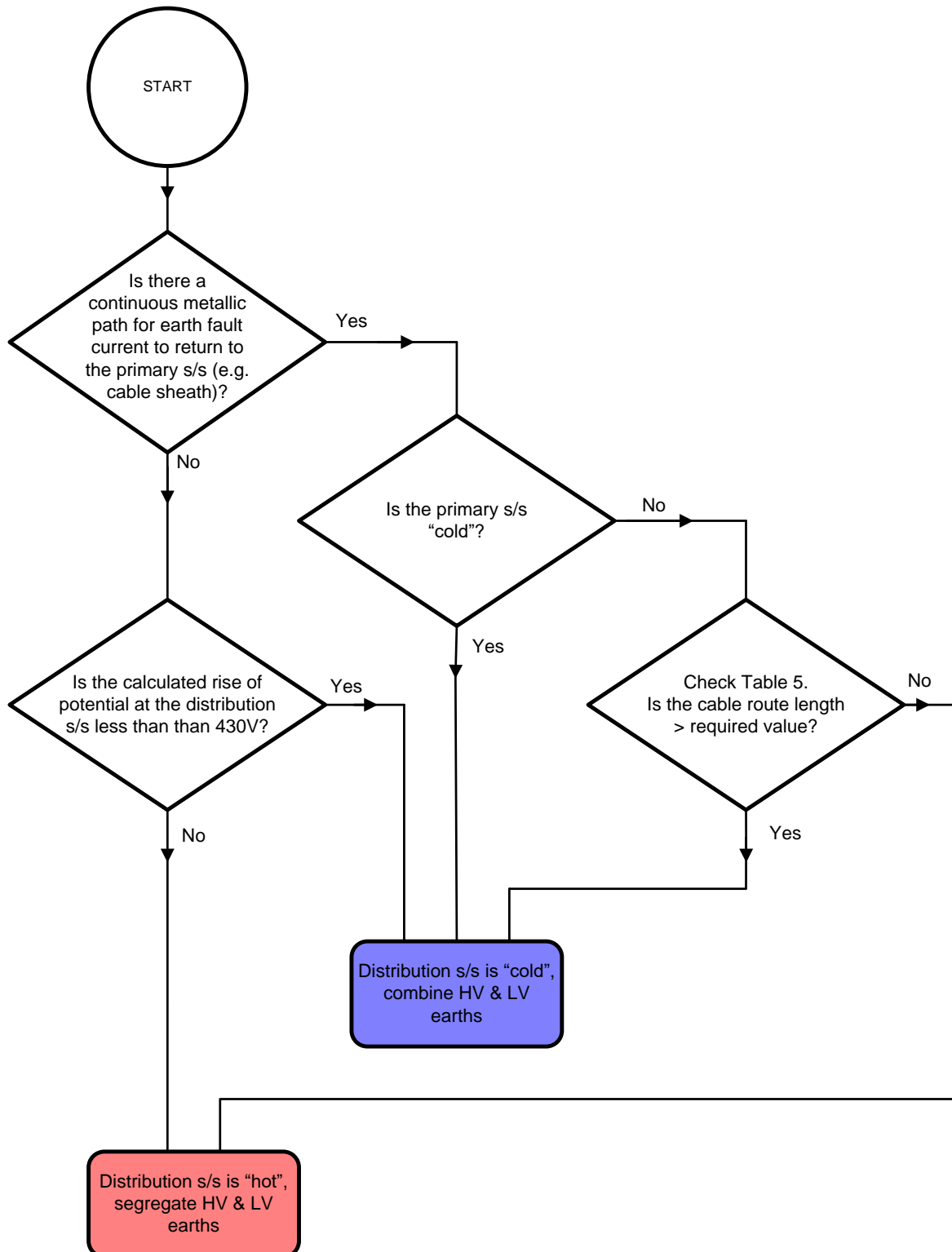
Figure 15: Process to Determine the Hot / Cold Status of a Distribution Substation
