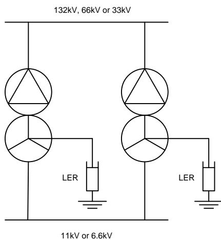
Figure 10: Resistance Earthing
