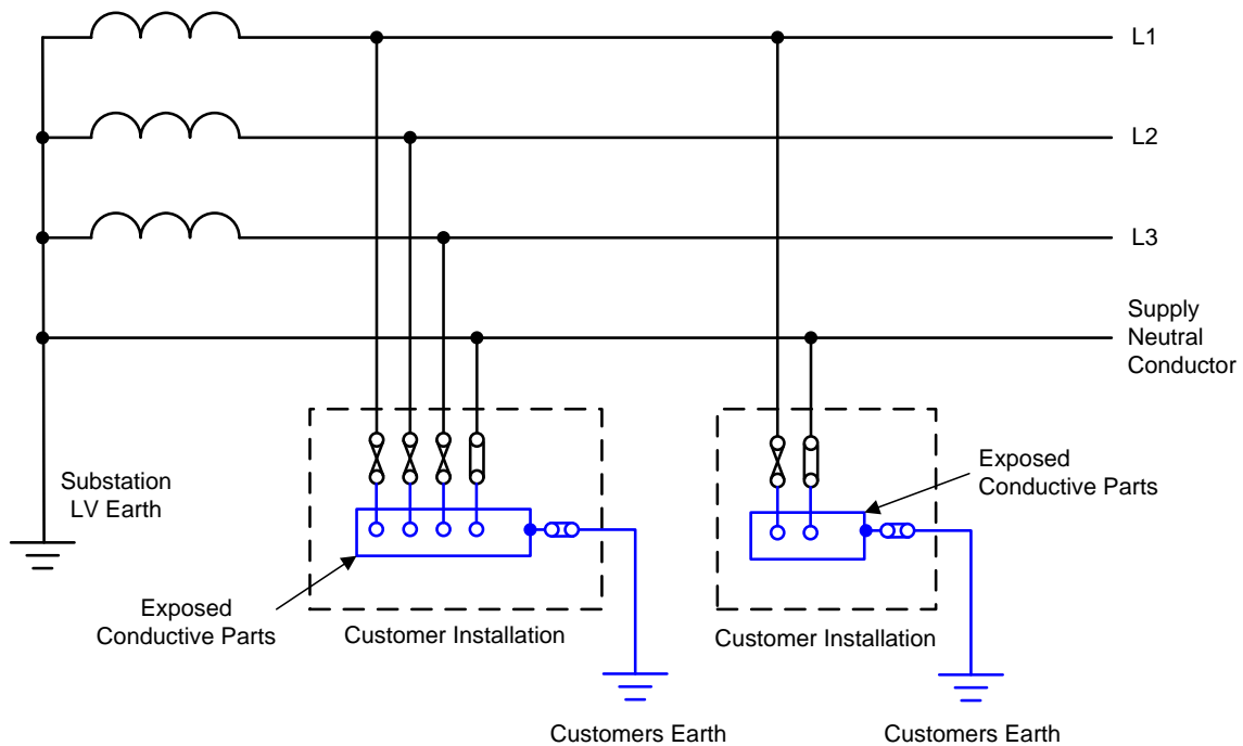
Figure 42: Direct Earthing
