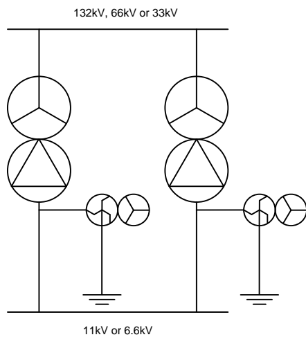
Figure 13: High Impedance Earthing
