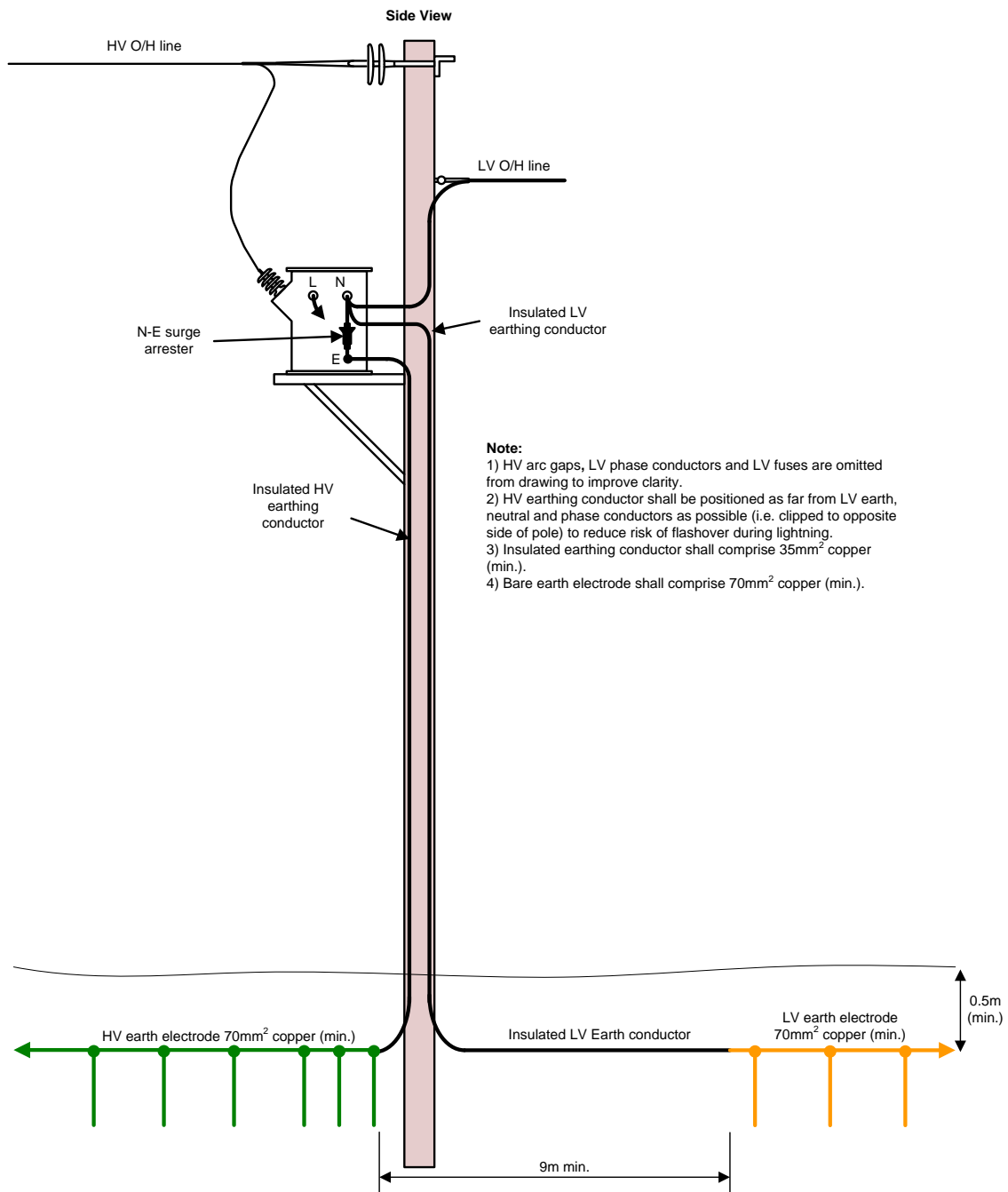
Figure 24: Segregating HV and LV Earthing at Pole Mounted Substations - LV earth connected at transformer pole - HV and LV overhead lines
