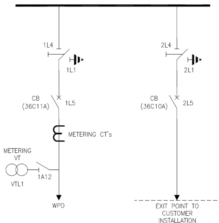
SINGLE CIRCUIT TEED CONNECTION
