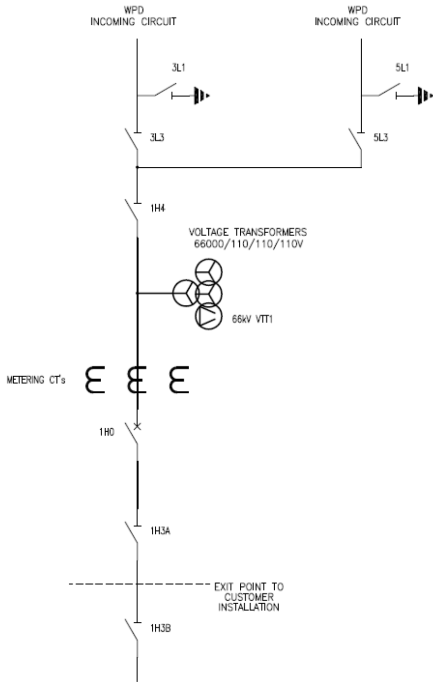
SINGLE CIRCUIT LOOPED CONNECTION
