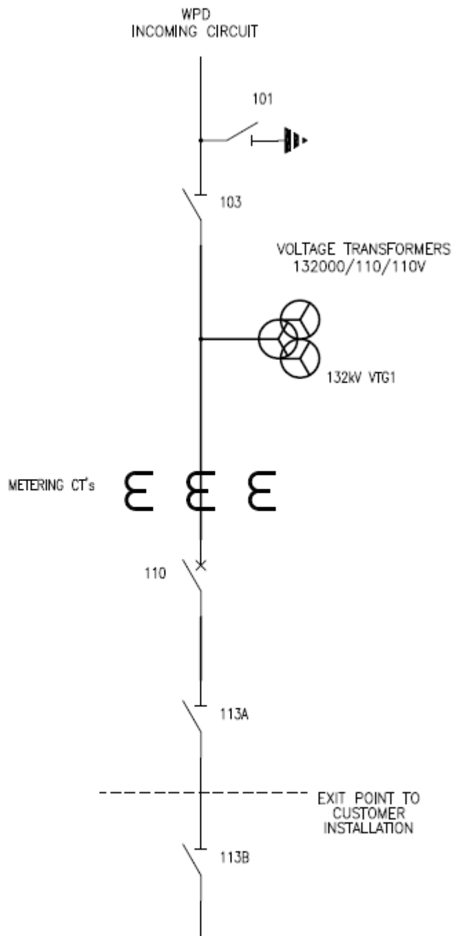
SINGLE CIRCUIT TEED CONNECTION
