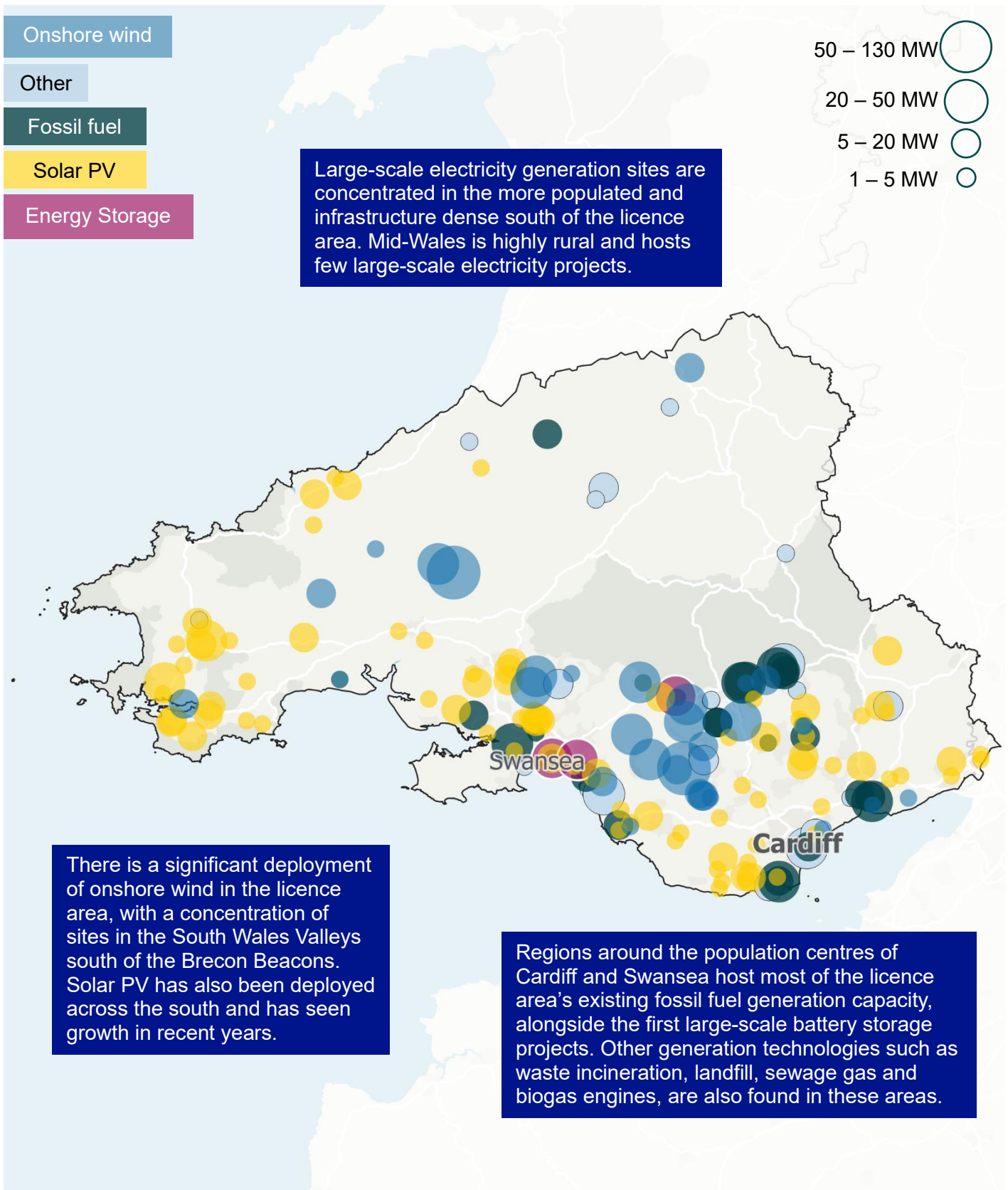
Figure 4: The NGED South Wales licence area, with the location of existing 'baseline' large-scale generation and storage sites
