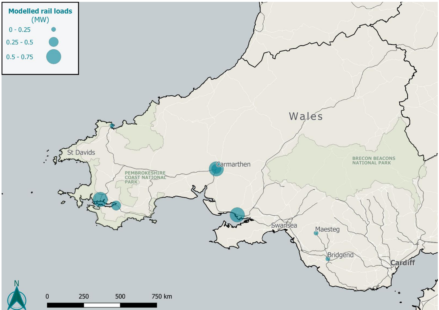
Map of additional rail sector loads on the distribution network in 2050. Size of circles represent the scale of capacity required.
